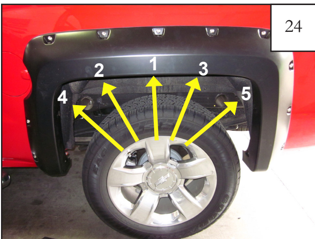
Install supplied self-tapping screws (Item 1) into pilot holes in the order indicated. TIGHTEN ALL SCREWS
